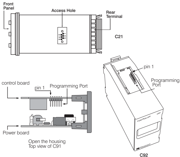
Figure 1.2 Programming Port Overview
