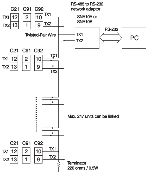
Figure 2.21 RS-485 Wiring
