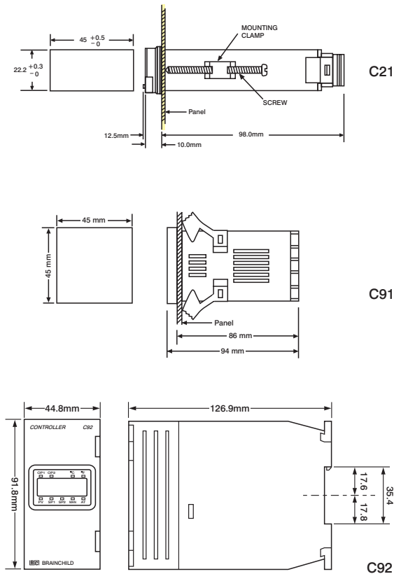
Figure 2.1 Mounting Dimensions
