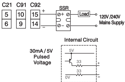
Figure 2.11 Output 1 Pulsed Voltage to Drive SSR
