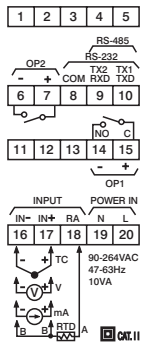
Figure 2.6 Rear Terminal Connection for C92
