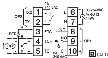
Figure 2.5 Rear Terminal Connection for C91
