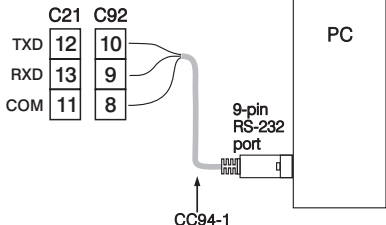
Figure 2.22 RS-232 Wiring
