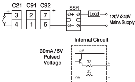
Figure 2.16 Output 2 Pulsed Voltage to Drive SSR
