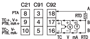
Figure 2.8 Sensor Input Wiring
