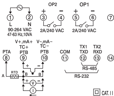
Figure 2.4 Rear Terminal Connection for C21
